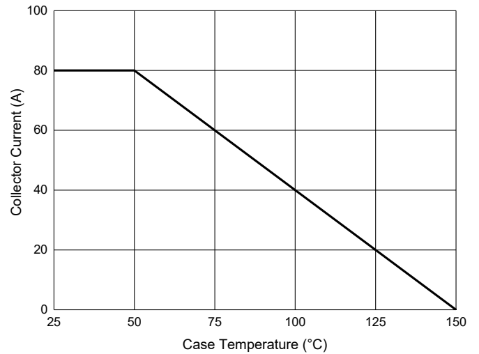
Fig. 10 - Collector Current Derating Curve
