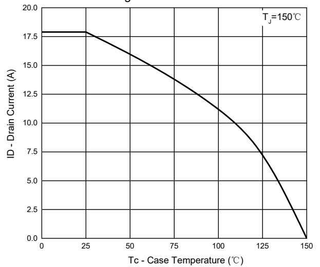
Fig. 10 - Drain Current
