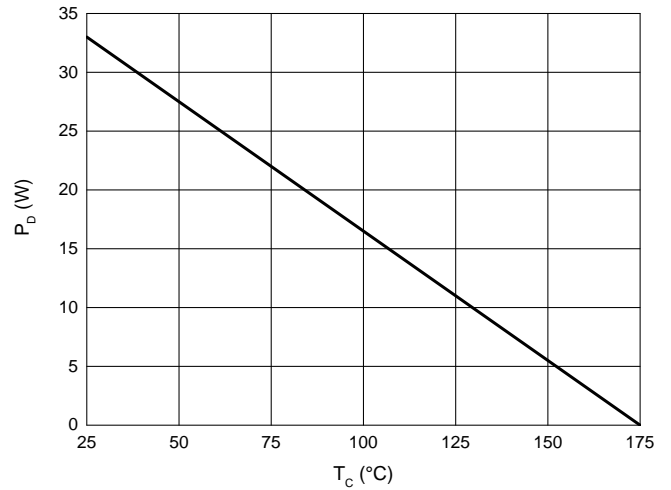
Fig. 6 - Power Derating
