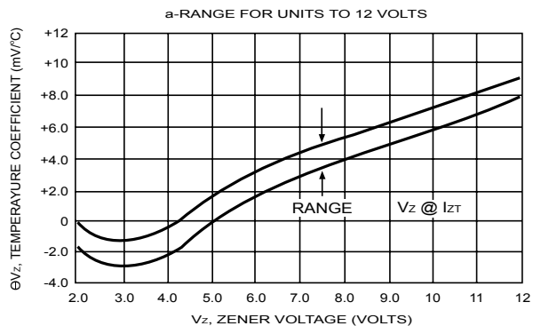
FIG.7- TEMPERATURE COEFFICIENTS
