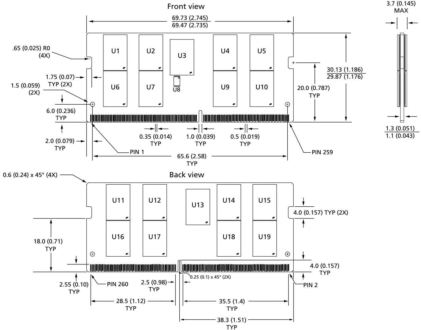
Figure 6: 260-Pin DDR4 SODIMM, R/C-G1 (PCB 2451)
