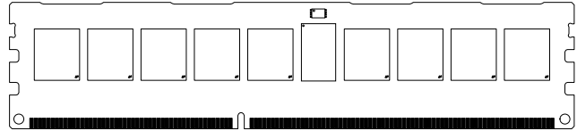
Figure 2: 240-Pin RDIMM (MO-269 R/C B1)
