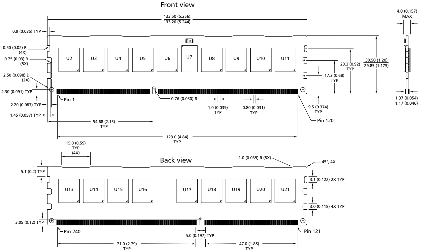
Figure 6: 240-Pin DDR3 RDIMM R/C B1 (PCB 1164, 1382)
