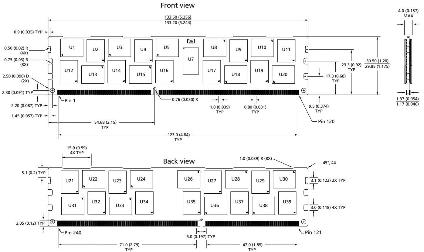
Figure 6: 240-Pin DDR3 RDIMM (R/C E2)
