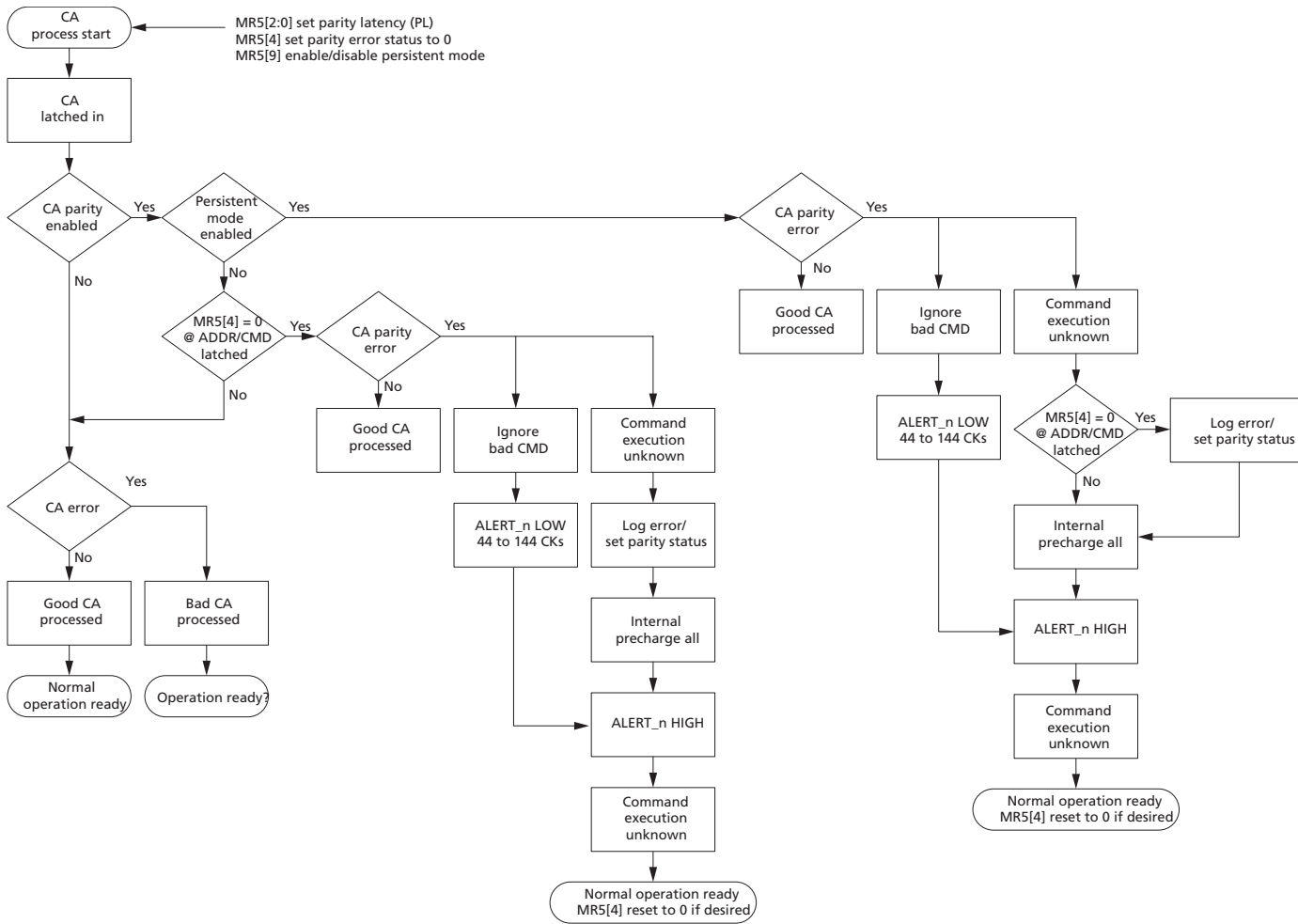
Figure 61: CA Parity Flow Diagram
