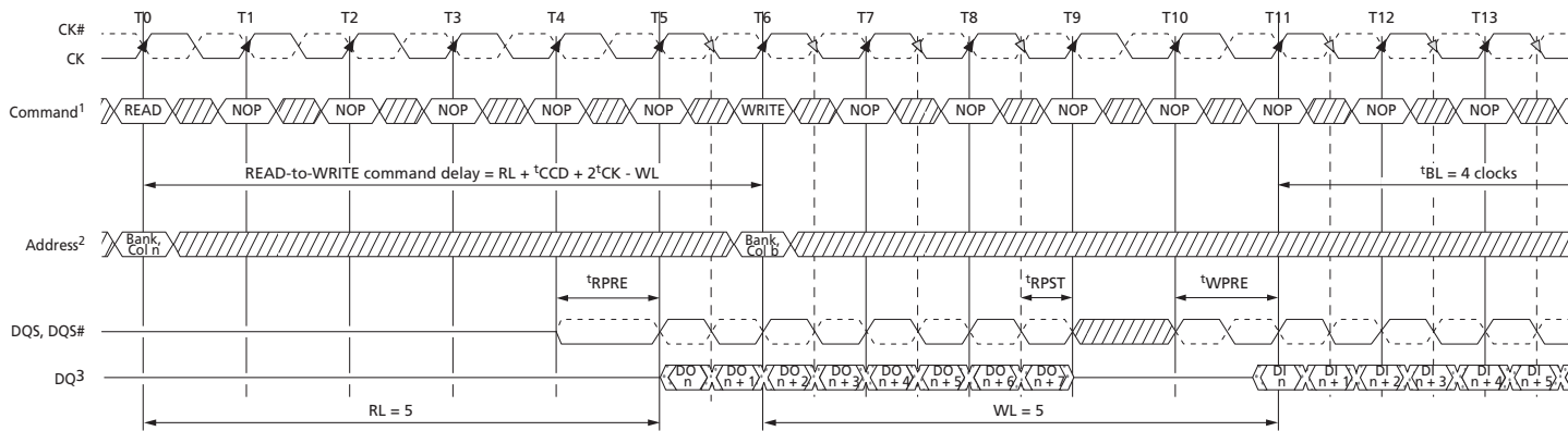
Figure 72: READ (BL8) to WRITE (BL8)
