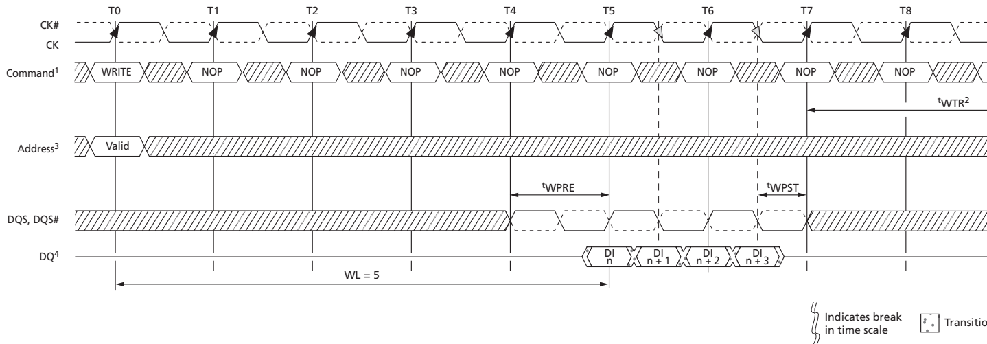
Figure 90: WRITE to READ (BC4 Mode Register Setting)
