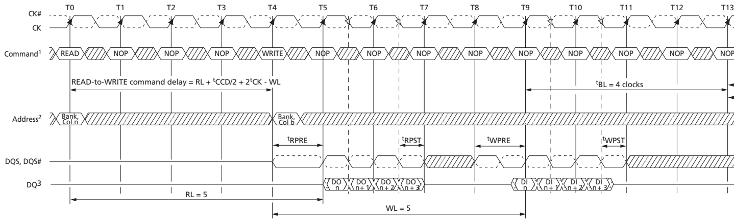
Figure 73: READ (BC4) to WRITE (BC4) OTF
