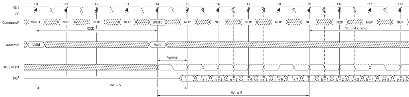
Figure 86: Consecutive WRITE (BL8) to WRITE (BL8)
