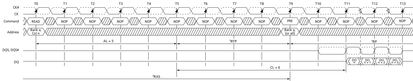
Figure 76: READ to PRECHARGE (AL = 5, CL = 6)
