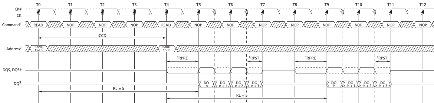
Figure 70: Consecutive READ Bursts (BC4)
