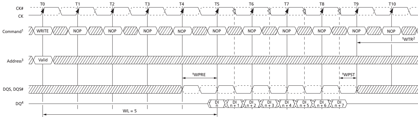
Figure 89: WRITE (BL8) to READ (BL8)
