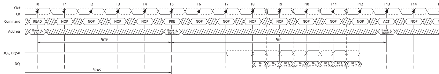
Figure 74: READ to PRECHARGE (BL8)
