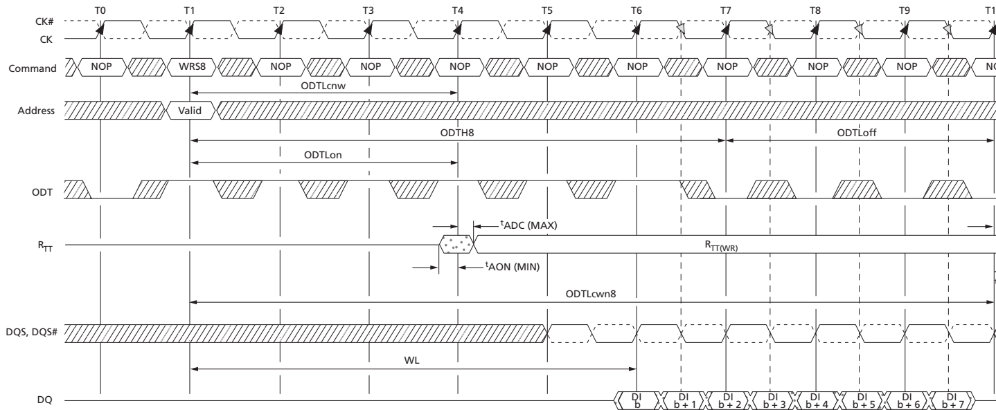
Figure 112: Dynamic ODT: ODT Pin Asserted Together with WRITE Command for 6 Clock Cycles, BL8
