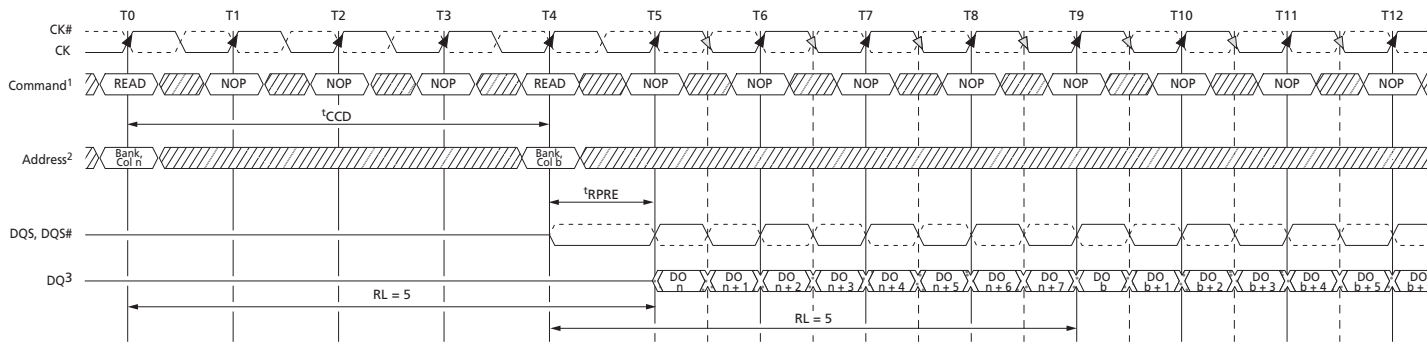
Figure 69: Consecutive READ Bursts (BL8)
