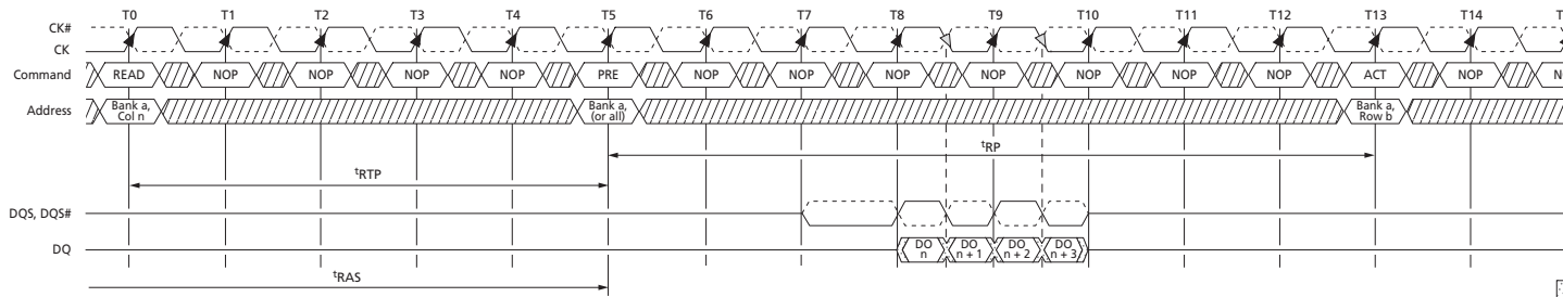
Figure 75: READ to PRECHARGE (BC4)
