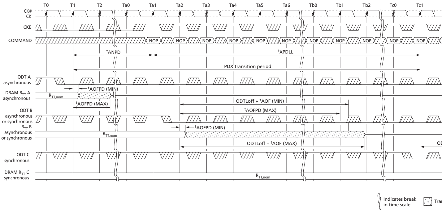
Figure 120: Asynchronous to Synchronous Transition During Precharge Power-Down (DLL Off) Exit
