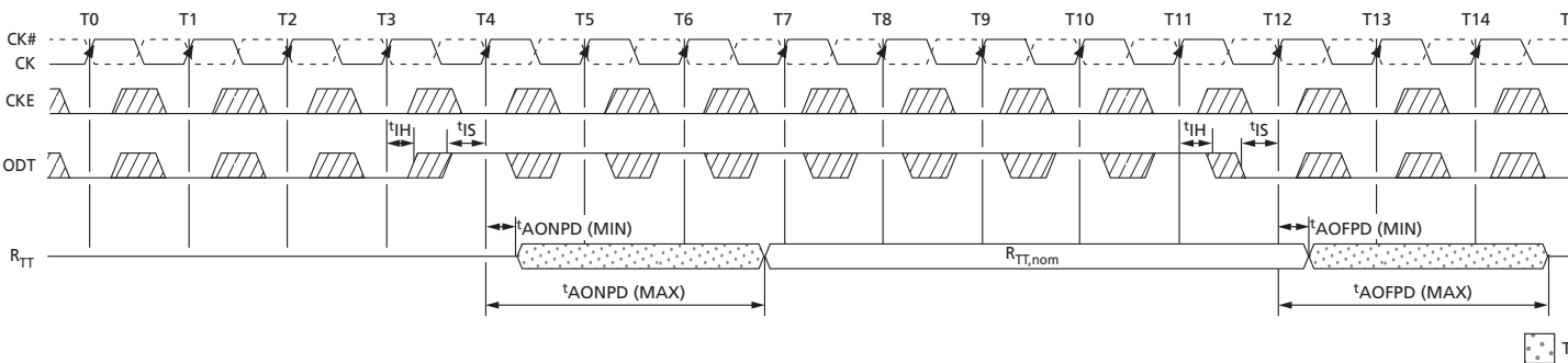
Figure 118: Asynchronous ODT Timing with Fast ODT Transition
