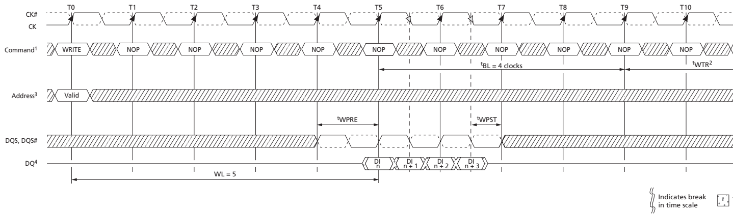
Figure 91: WRITE (BC4 OTF) to READ (BC4 OTF)
