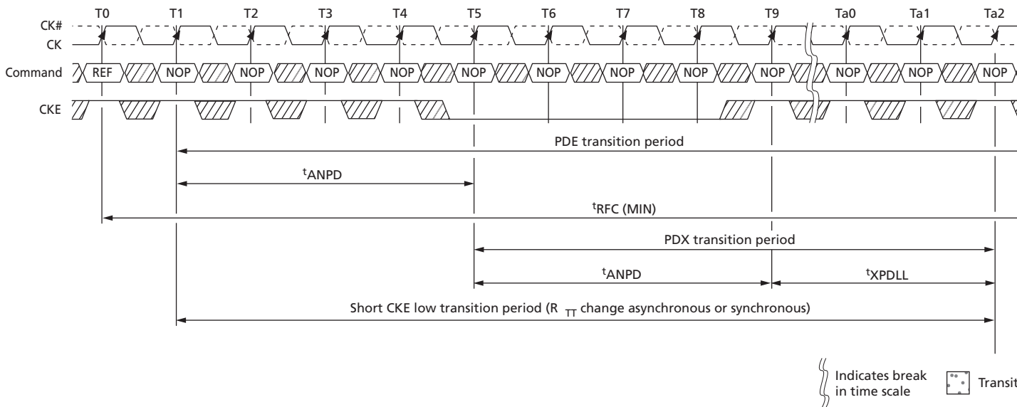
Figure 121: Transition Period for Short CKE LOW Cycles with Entry and Exit Period Overlapping
