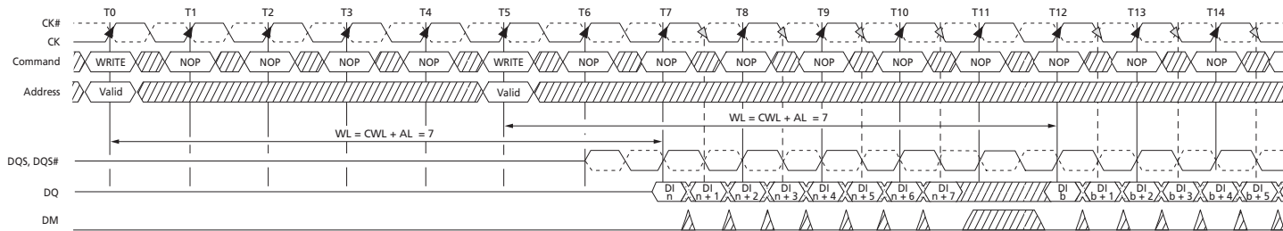
Figure 88: Nonconsecutive WRITE to WRITE
