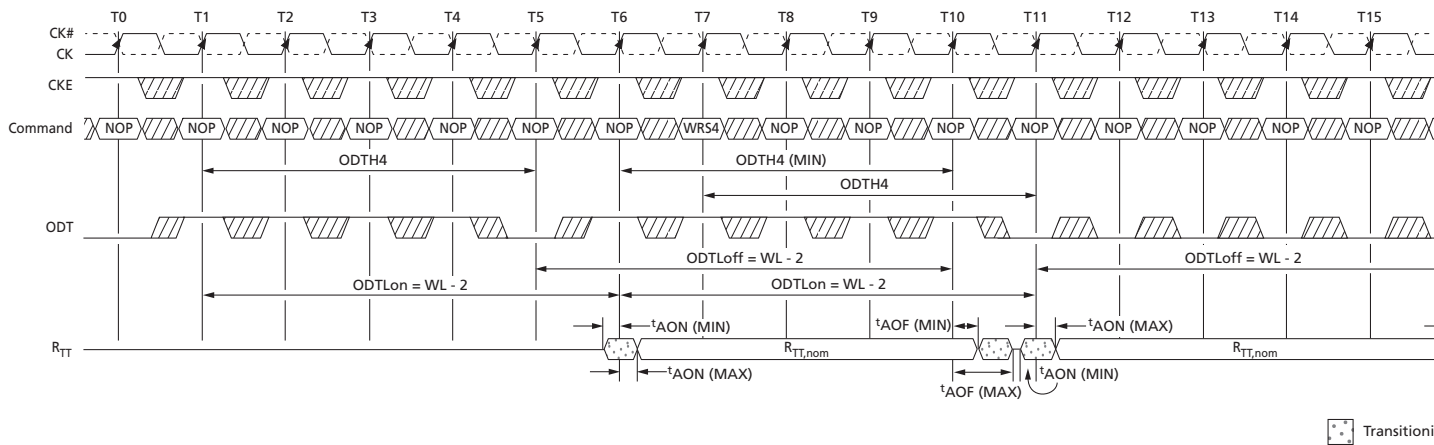
Figure 116: Synchronous ODT (BC4)
