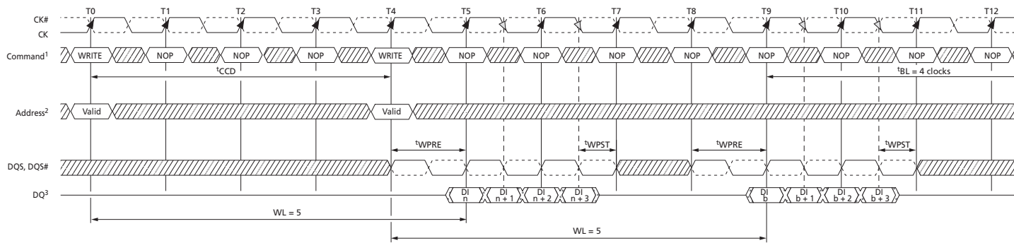
Figure 87: Consecutive WRITE (BC4) to WRITE (BC4) via OTF
