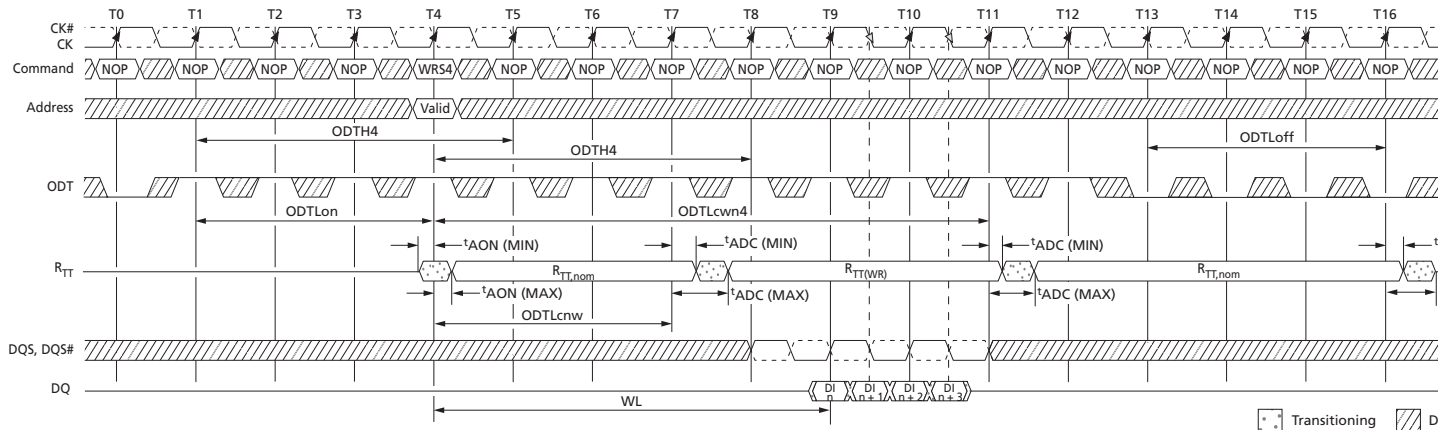
Figure 110: Dynamic ODT: ODT Asserted Before and After the WRITE, BC4
