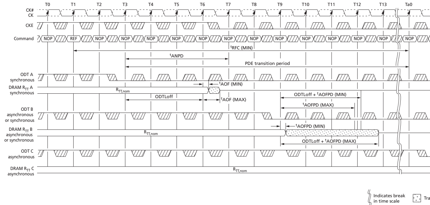
Figure 119: Synchronous to Asynchronous Transition During Precharge Power-Down (DLL Off) Entry
