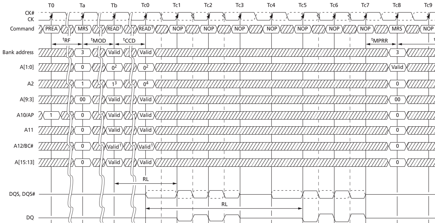
Figure 64: MPR System Read Calibration with BC4: Upper Nibble, Then Lower Nibble
