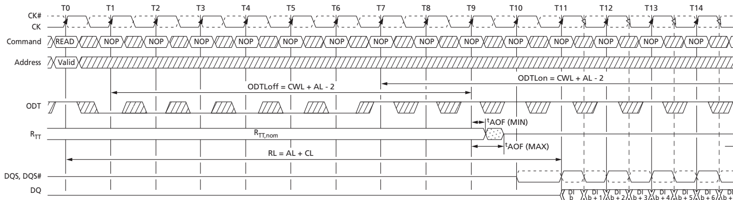
Figure 117: ODT During READs
