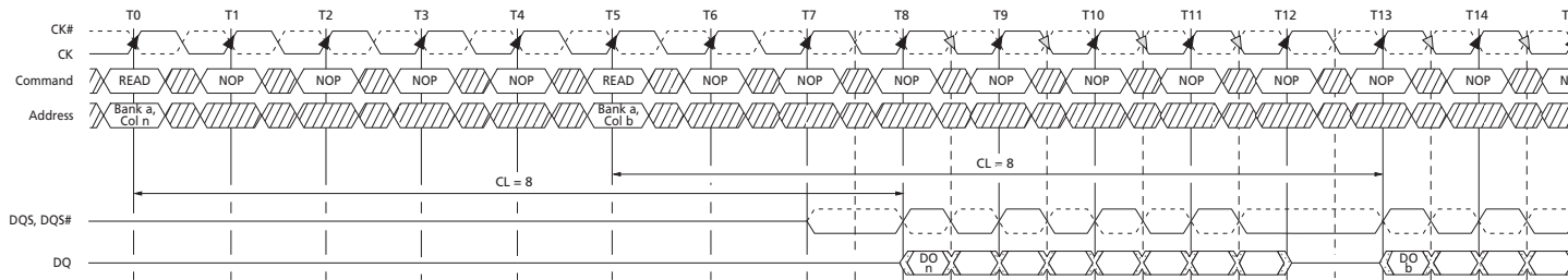
Figure 71: Nonconsecutive READ Bursts
