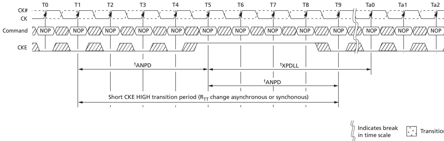
Figure 122: Transition Period for Short CKE HIGH Cycles with Entry and Exit Period Overlapping
