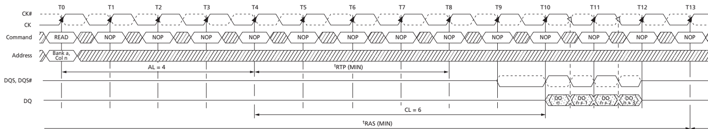
Figure 77: READ with Auto Precharge (AL = 4, CL = 6)
