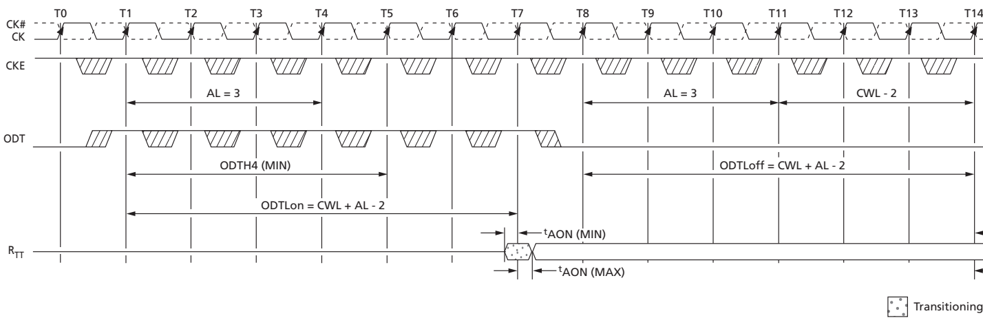
Figure 114: Synchronous ODT
