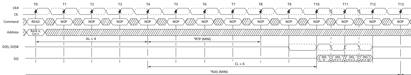
Figure 76: READ with Auto Precharge (AL = 4, CL = 6)
