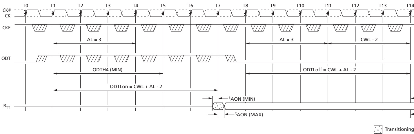
Figure 116: Synchronous ODT
