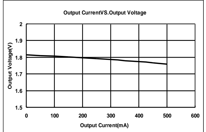
ME6211C18M5G
