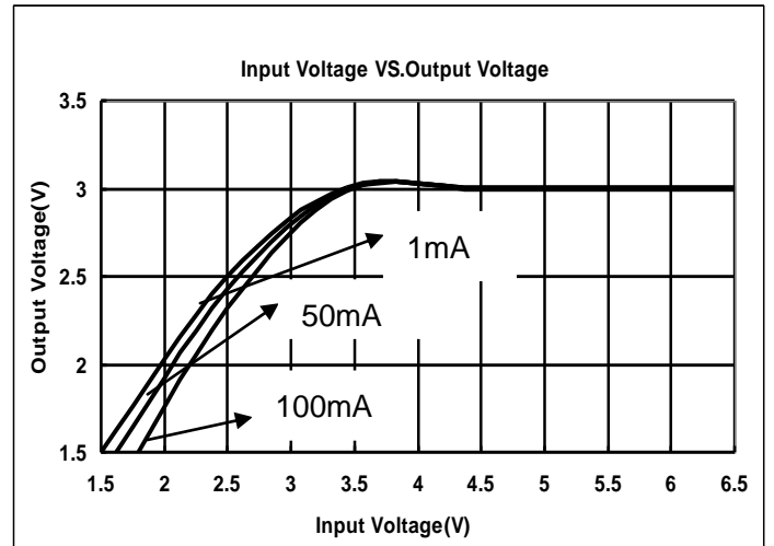
ME6211C30M5G
