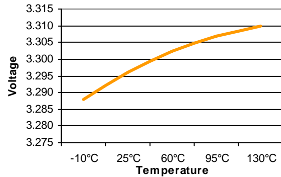
VOLTAGE OVER TEMPERATURE
