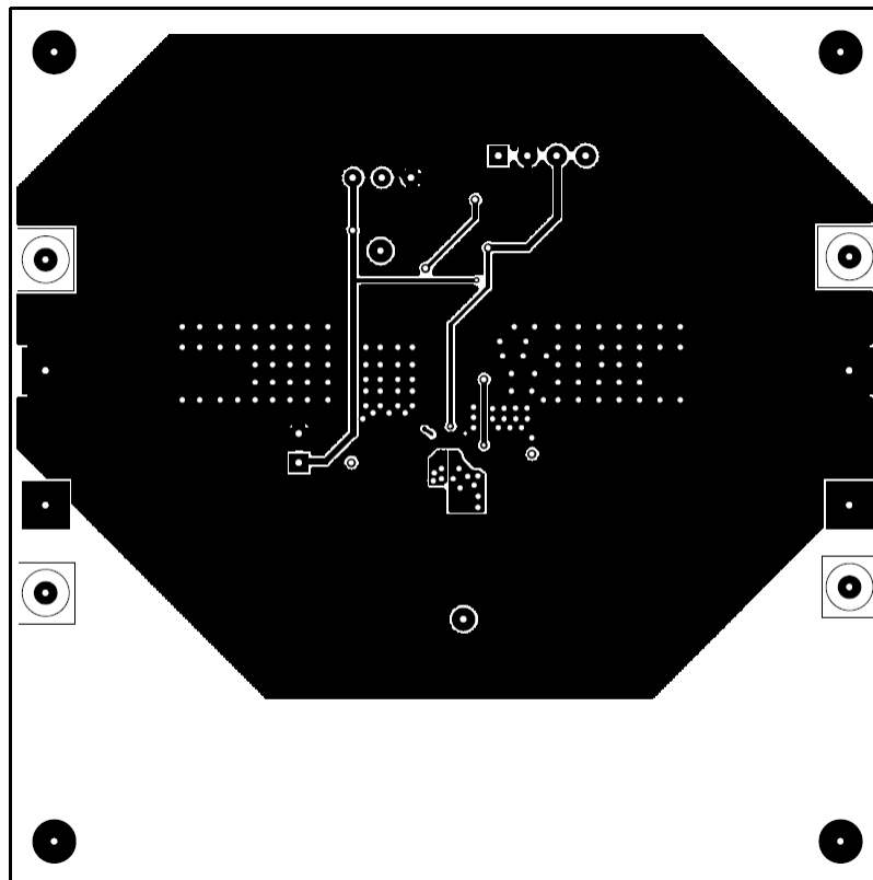
Figure 7: Layout recommendation (BOTTOM layer)
