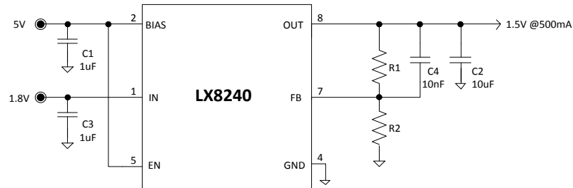
Figure 20 · Typical Application
