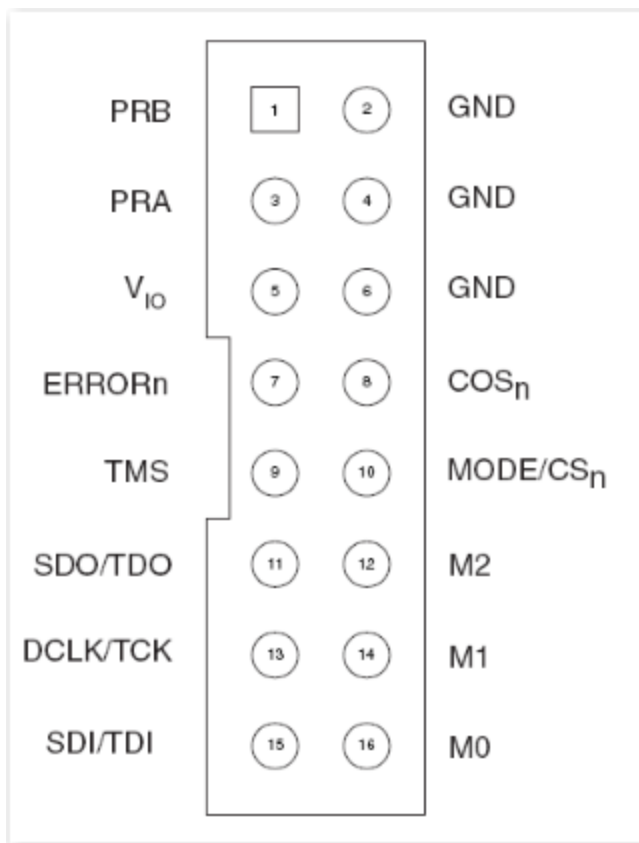
Figure 1 · Silicon Explorer II Probe Connector Pin-Out Table 5 · Matching Probe Pins to Device Pins 1
