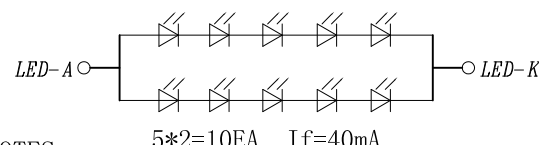
LED CIRCUIT DIAGRAM:
