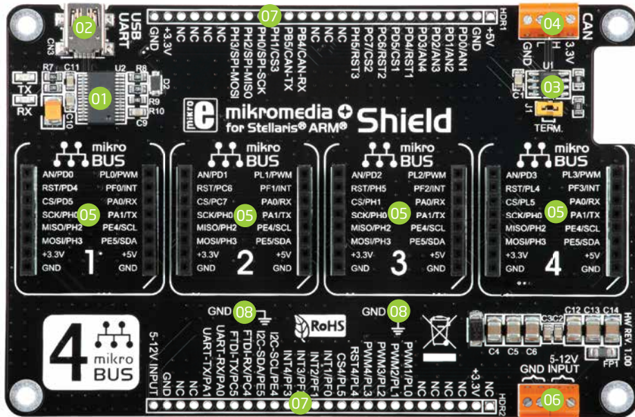
Figure 1-1: mikromedia+ shield
