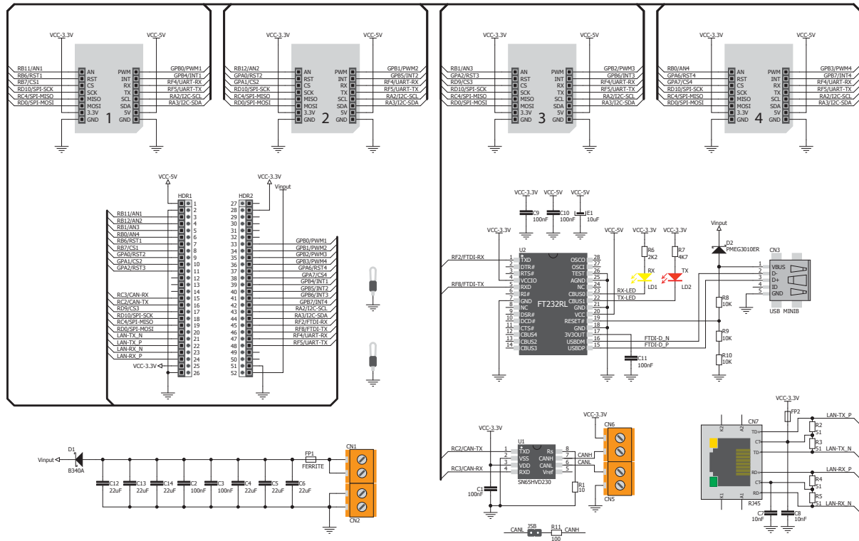
Figure 1-2: mikromedia+ SHIELD for PIC32MX7® schematic
