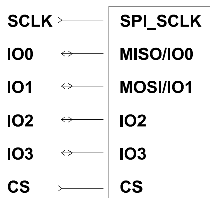
Figure 5. QSPI interface connection
