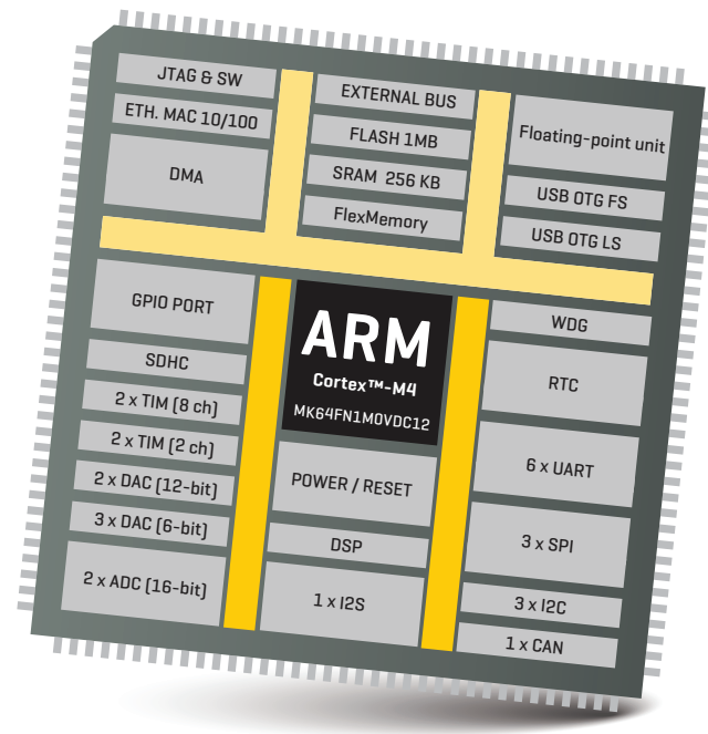
Figure 1: Kinetis MK64FN1M0VDC12 MCU block schematic
