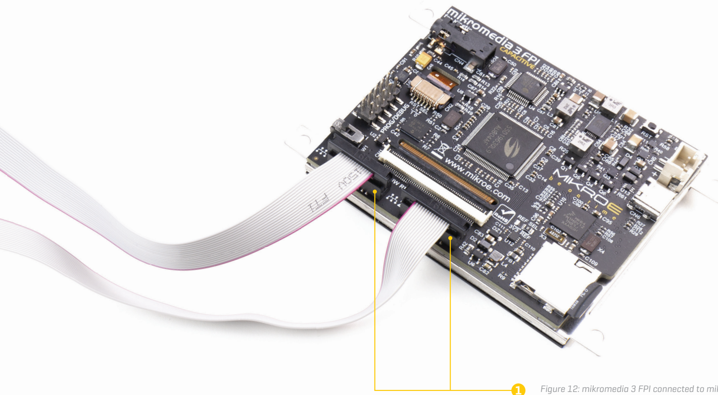
Figure 12: mikromedia 3 FPI connected to mikroBUS Shuttle view
