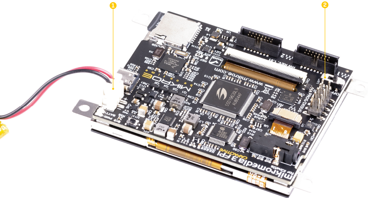
Figure 8: Battery power supply connection
