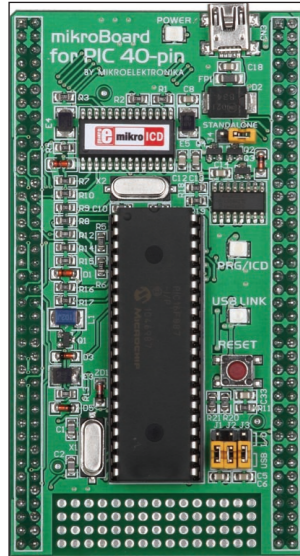
Figure 2-1: mikroBoard for PIC 40-pin
