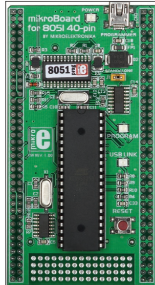
Figure 2-2: mikroBoard for 8051 40-pin
