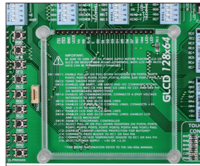
Figure 15-2: GLCD connector
