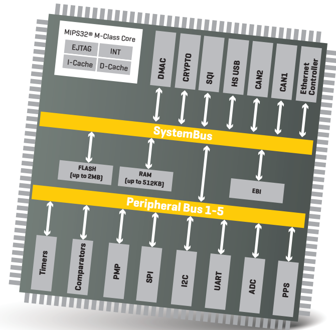
Figure 1: PIC32MZ2048EFH100 MCU block schematic
