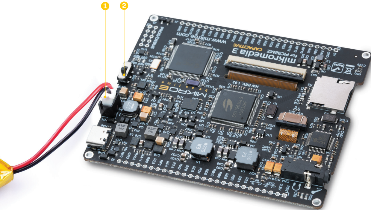
Figure 8: Battery power supply connection
