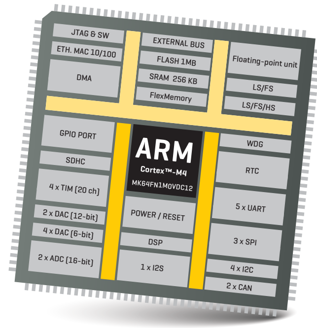
Figure 1: MK66FX1MOV1Q18 MCU block schematic
