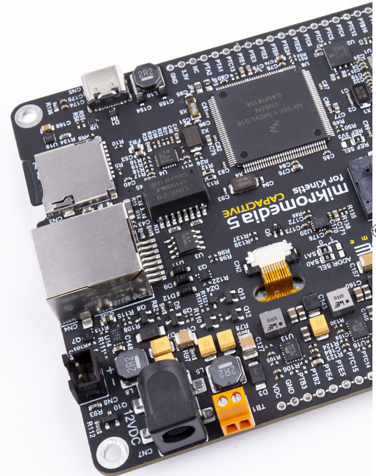
Figure 15: mikromedia 5 back view
