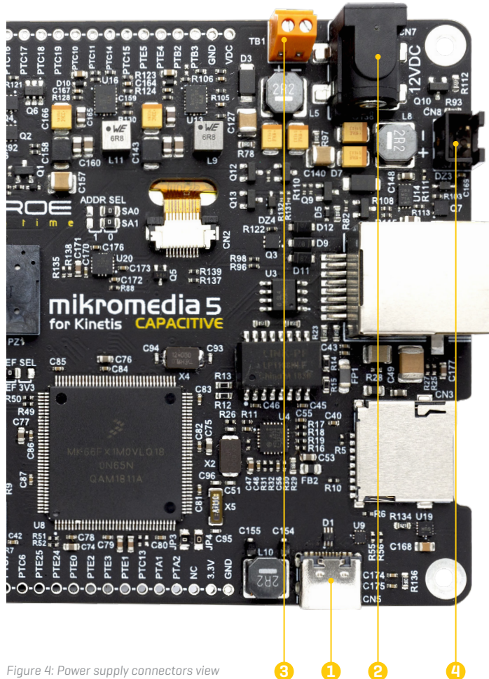
Figure 4: Power supply connectors view
