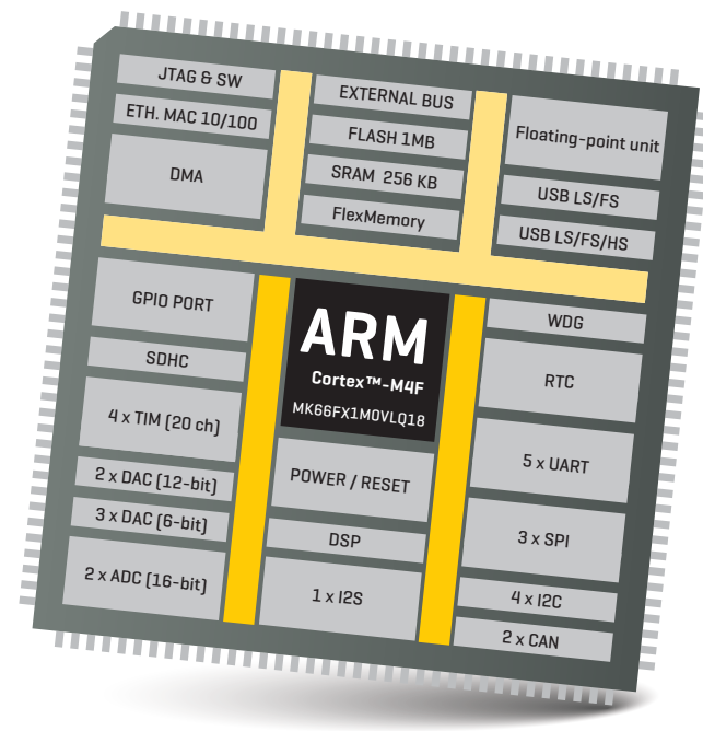
Figure 1: MK66FX1MOVLQ18 MCU block schematic
