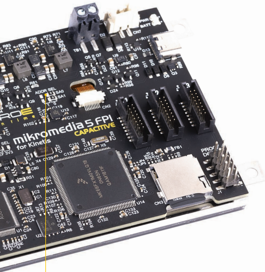
Figure 16: mikromedia 5 FPI back view
