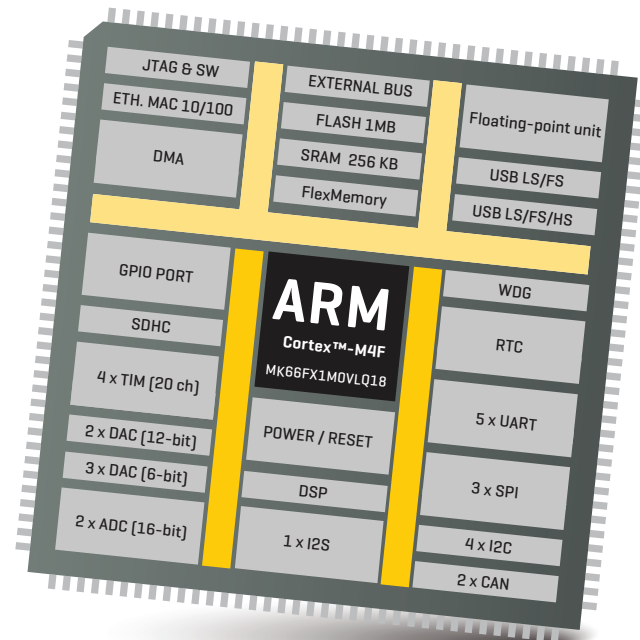
Figure 1: Kinetis MK66FX1MOV1Q18 MCU block schematic
