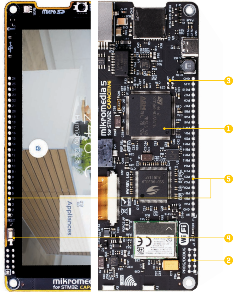
Figure 2: Front and back partial view
