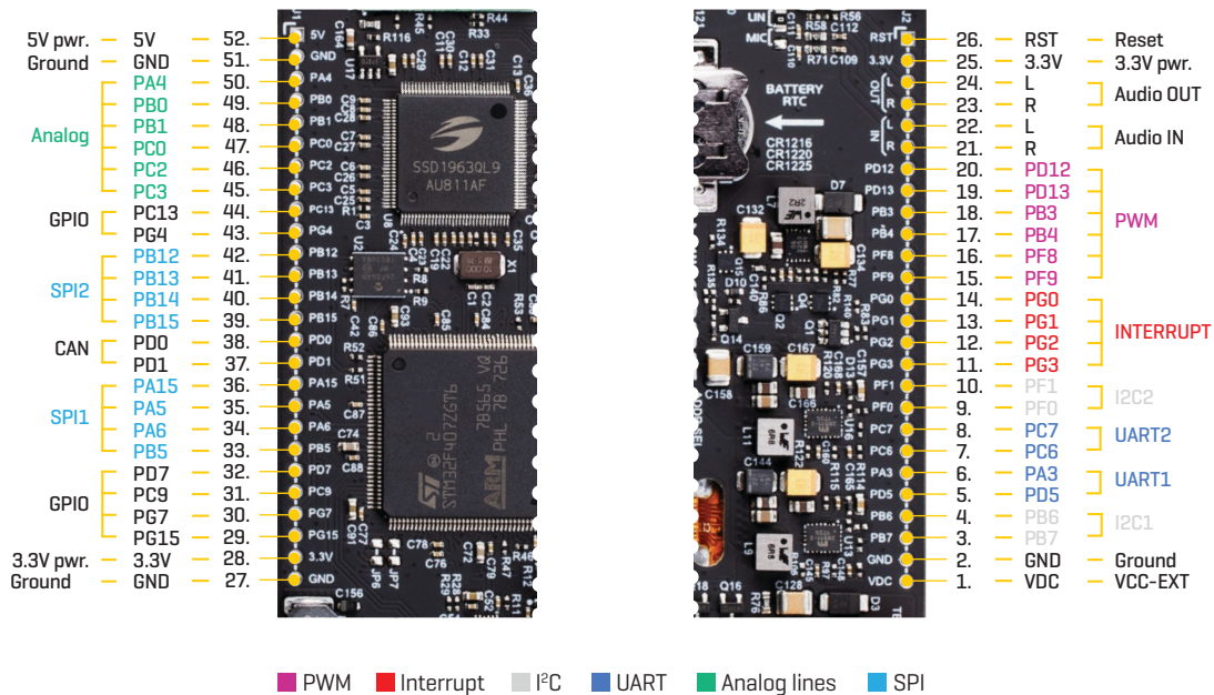
Figure 14: 1x26 pin header view
