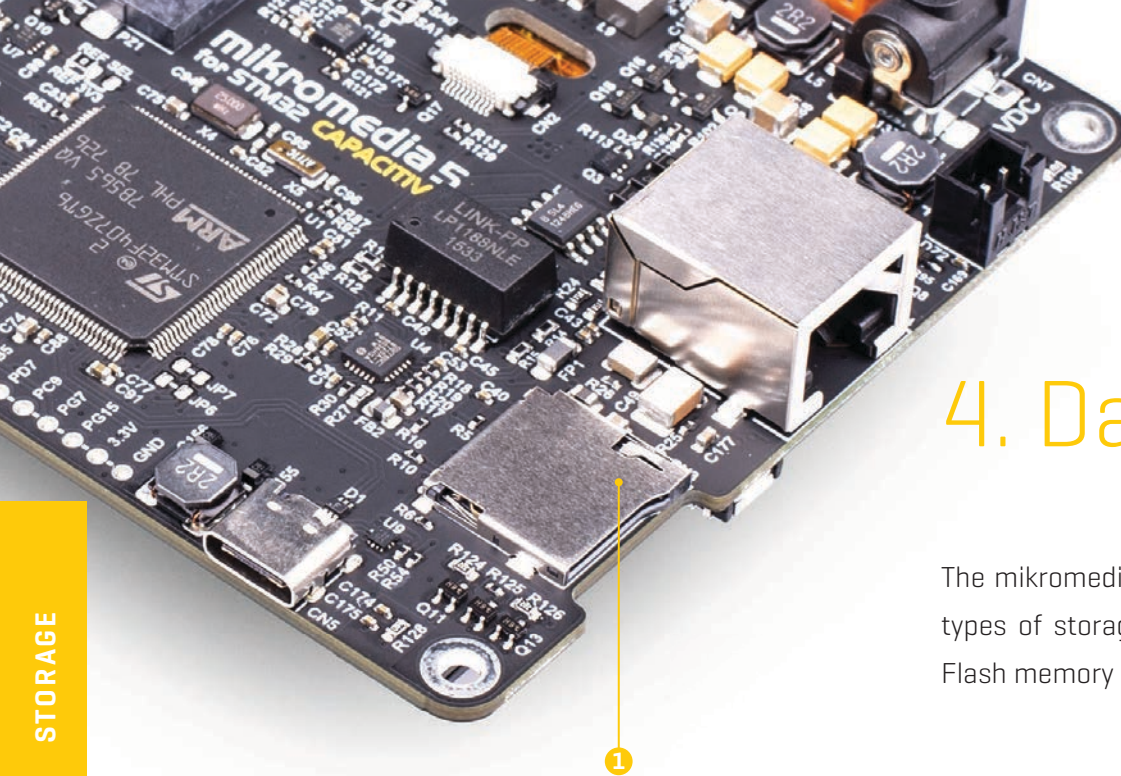
Figure 10: microSD card slot view
