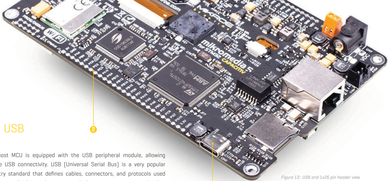
Figure 13: USB and 1x26 pin header view
