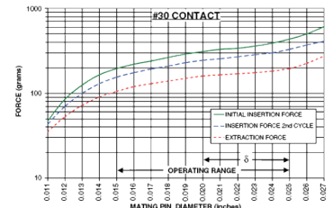
CONTACT MATERIAL BERYLLIUM COPPER Alloy 172, Heat Treated
