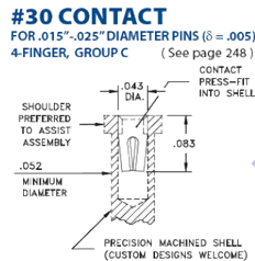
CONTACT MATERIAL BERYLLIUM COPPER Alloy 172, Heat Treated
