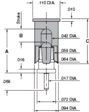
806-22-001-10-00X191 Removable Pick & Place Cap, Through-hole mount
