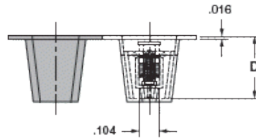
806-22-001-10-00X191 Removable Pick & Place Cap, Through-hole mount
