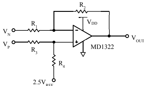
Figure 25. Differential Amplifier
