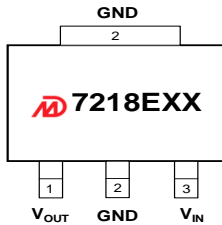
SOT89-3L(E_Type) Top View
