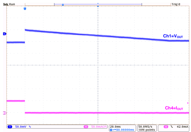
Load Transient at V_{OUT}=3.3V : ( I_{OUT}=50mA-0mA )
