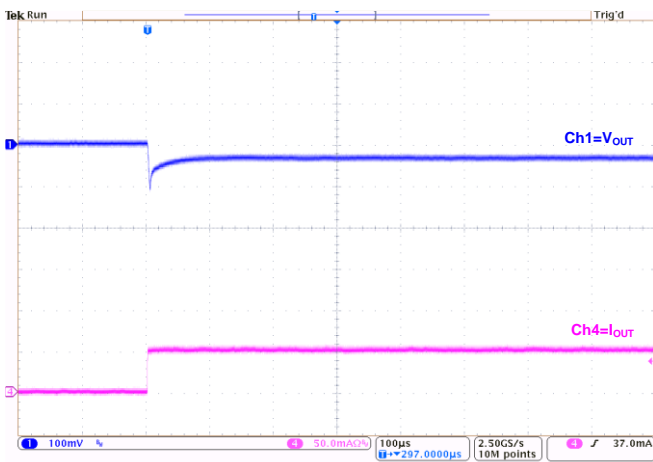
Load Transient at V_{OUT}=3.3V : ( I_{OUT}=0mA-50mA )
