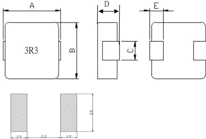
PCB Layout
