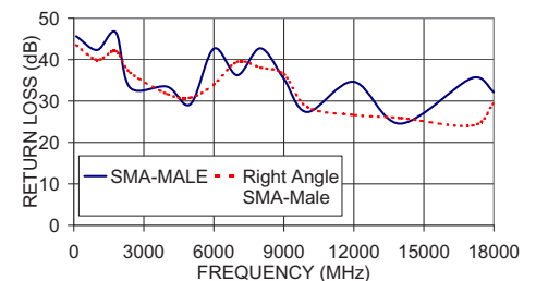
086-10SMRSM+ RETURN LOSS
