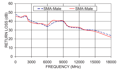
141-20SM+ RETURN LOSS
