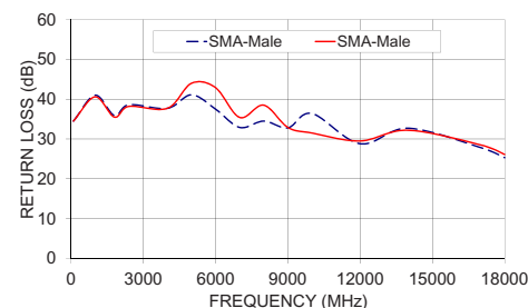
141-22SM+ RETURN LOSS
