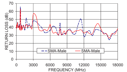
141-24SM+ RETURN LOSS
