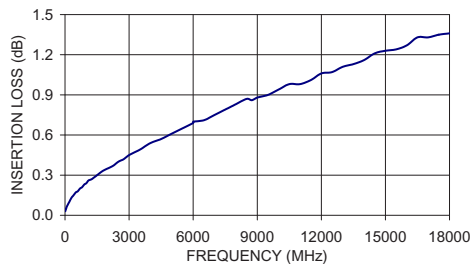
141-24SM+ INSERTION LOSS
