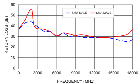
141-60SM+ RETURN LOSS
