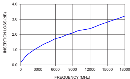
141-60SM+ INSERTION LOSS
