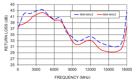
141-72SM+ RETURN LOSS
