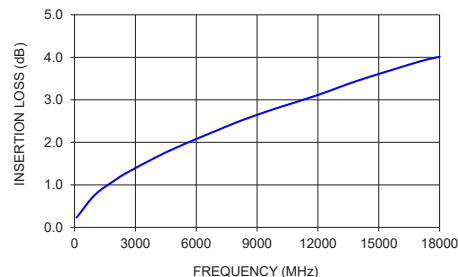
141-72SM+ INSERTION LOSS
