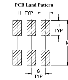
Suggested Layout, Tolerance to be within ±.002
