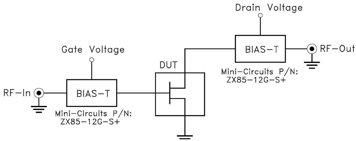
Fig 1. Block Diagram of Test Circuit used for characterization. (DUT soldered on Mini-Circuits Test Board TB-154)
