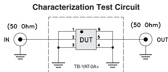
Fig 1. Block diagram of Test Circuit used for characterization, Test board TB-YAT-0A+ Conditions: Attenuation, VSWR: Pin=-10 dBm
