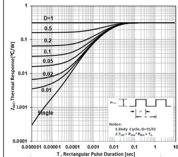
Figure 3a Max Thermal Impedance (TO-247&TO-3PN)
