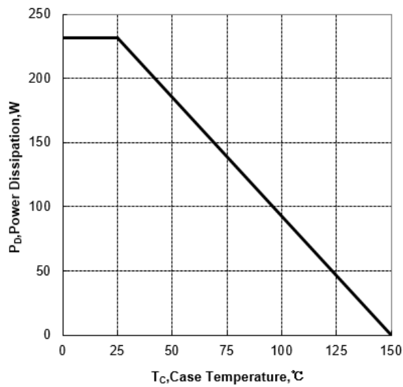
Figure 2b Power Dissipation (TO-220)
