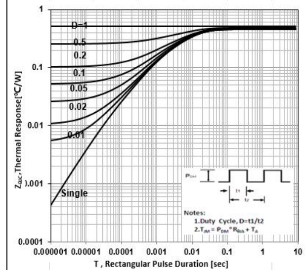
Figure 3b Max Thermal Impedance (TO-220)
