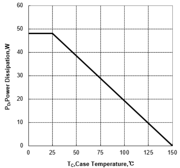
Figure 2c Power Dissipation (TO-220F)
