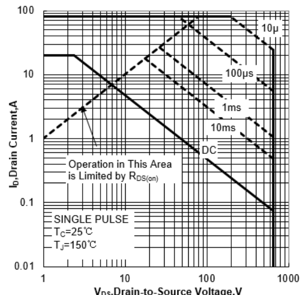
Figure 1c Safe Operating Area (TO-220F)
