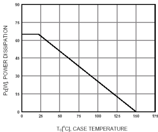
Figure 5. Power Derating
