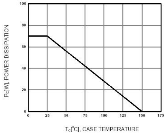
Figure 4. Power Derating
