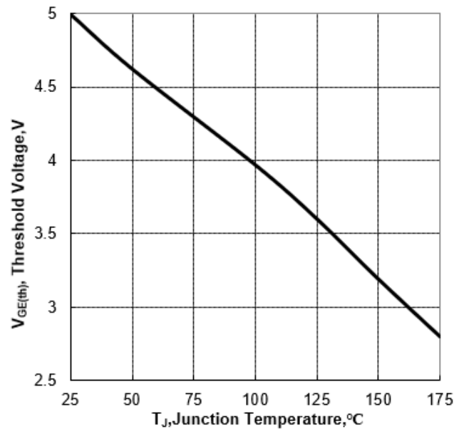
Figure 8. Typical Gate-Emitter Threshold Voltage vs Junction Temperature
