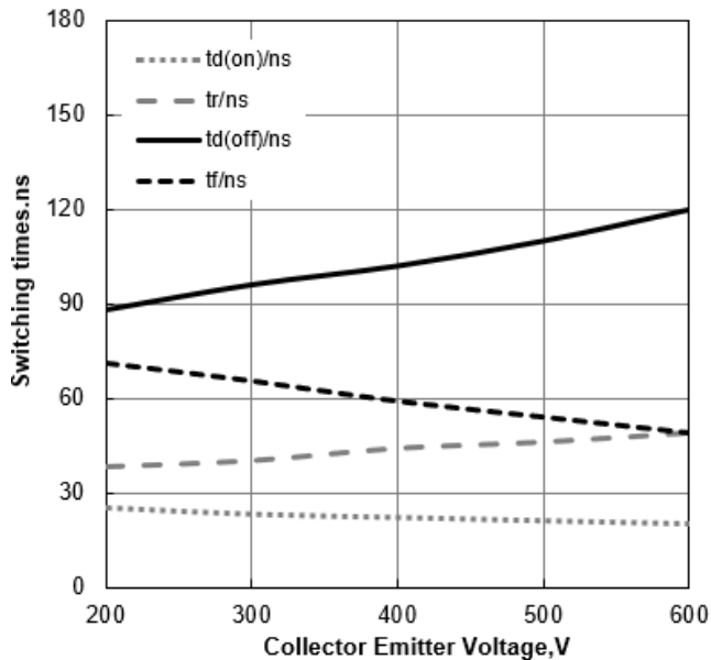
Figure 15. Typical Switching Times vs V CE (T J =25°C, V GE =15/0V, I C =50A)
