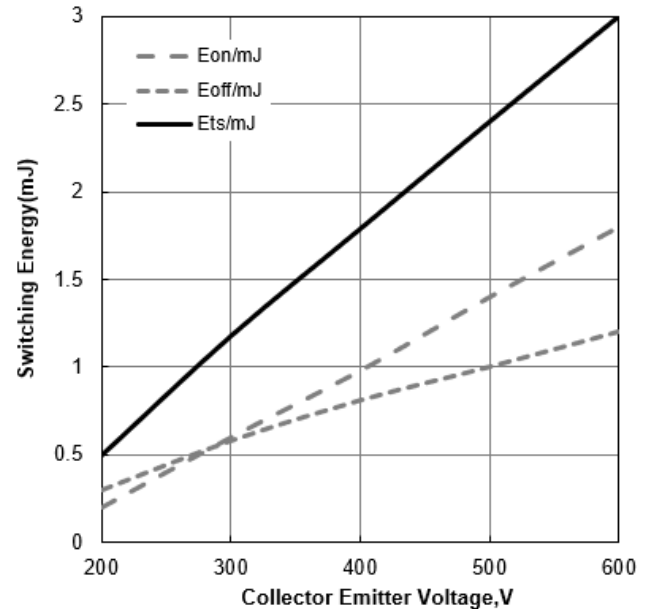
Figure 16. Typical Switching Energy vs V CE (T J =25°C, V GE =15/0V, I C =50A)
