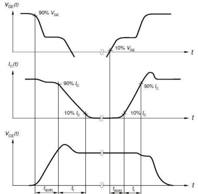
Figure 28. Definition of switching times
