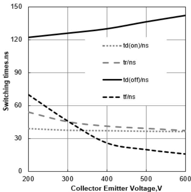
Figure 19. Typical Switching Times vs VCE (T J =25°C, V GE =15/0V, I C =60A)
