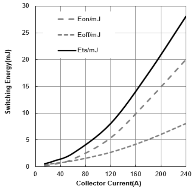
Figure 18. Typical Switching Energy vs Collector Current (T J =25°C, V CE =400V, V GE =15/0V)
