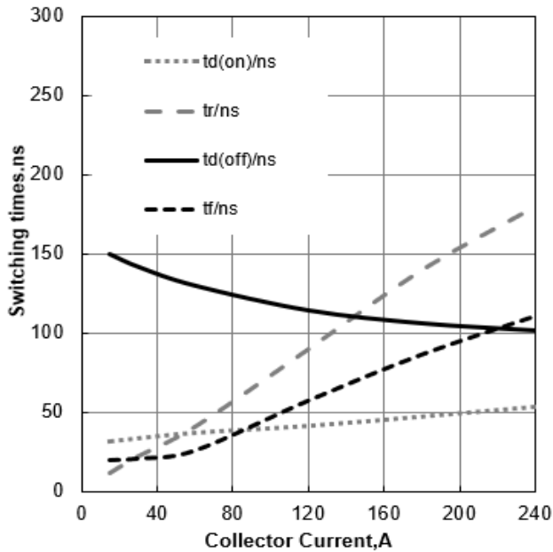
Figure 17. Typical Switching Times vs Collector Current (T J =25°C, V CE =400V, V GE =15/0V)
