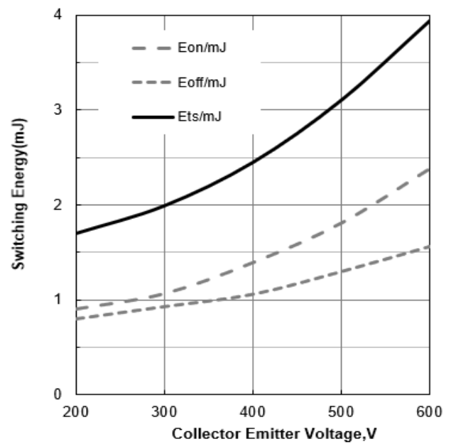
Figure 20. Typical Switching Energy vs VCE (T J =25°C, V GE =15/0V, I C =60A)
