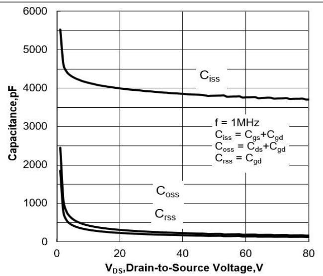
Figure 8 Capacitance Characteristics
