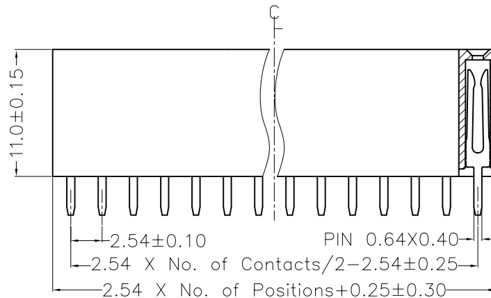
SECTION: A-A
